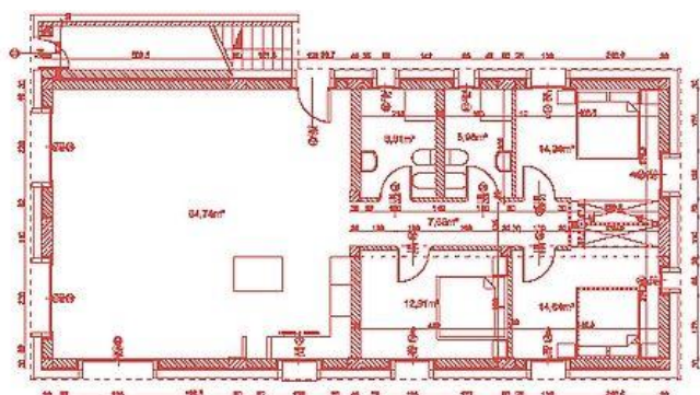
PARTER
