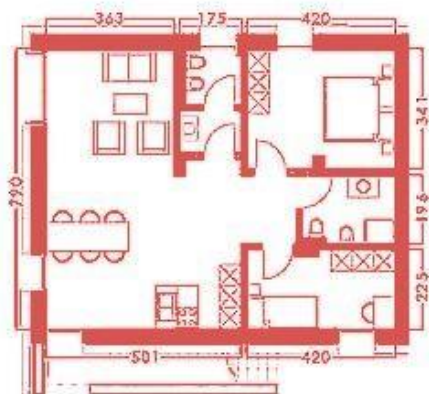
PARTER
