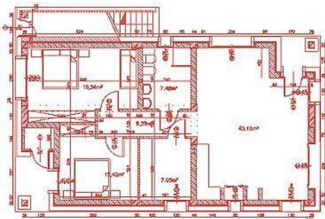
PARTER
